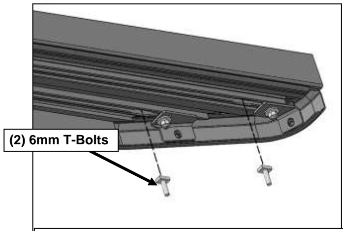
(Fig 4) Insert (6) T-Bolts into the channels in the bottom of the Running Board, (3) per channels
