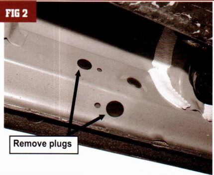
(Fig 2) Remove plugs from mounting locations as necessary
