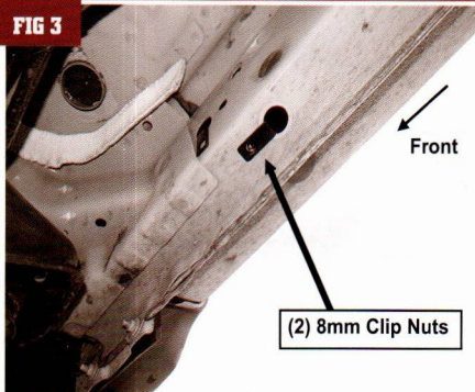
(Fig 3) Slide 8mm Clip Nut into large hole and over small hole
