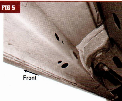
(Fig 5) Remove rubber plugs from the Passenger/Right center mounting location
