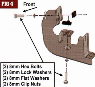
(Fig 4) Attach (1) Passenger/Right Mounting Bracket to the Clip Nuts
