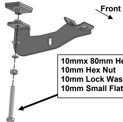
(Fig 12A) Assemble passenger/right Center Mounting Bracket with Support Pad
