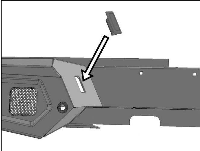
(Fig 13) Remove light from plastic mount. Push license plate light into Bumper
