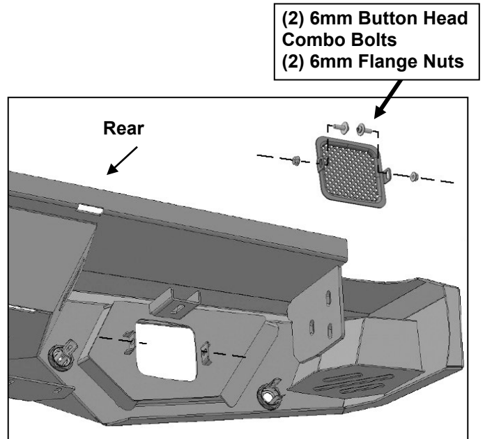
(Fig 12) Remove screens for additional access or to clear lights as needed
