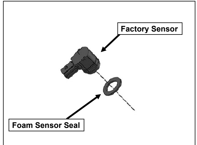
(Fig 10) Remove factory seal. Push Foam Seal onto end of sensor
