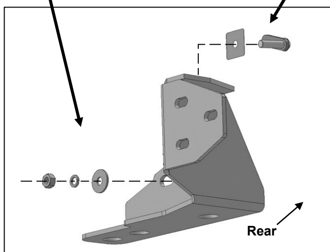
(Fig 7) Attach driver/left Mounting Bracket to Bolt Plate. Reuse factory hex bolts to attach bumper reinforcement or receiver hitch to bottom of Brackets and frame
