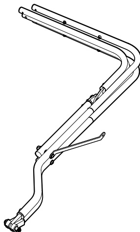
Bow Stack - Passenger Side Part #573.09 Qty.1
