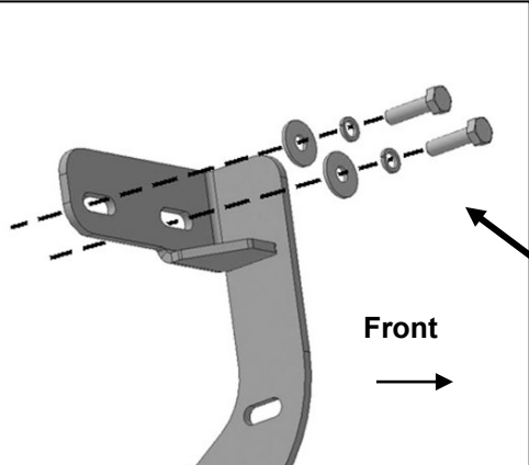
(Fig 10) Driver side front-models with factory installed threaded inserts. Bolt Plate not required
