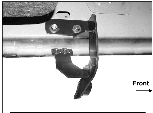
(Fig 14) Attach Driver/Left center Bracket
