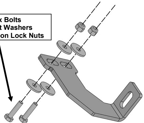
(Fig 6) Attach (1) Driver/Left Support Bracket to the pinch trim
