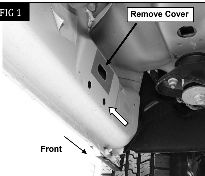
(Fig 1) 2009-mid 2015 front mounting location (No factory holes in pinch weld 2009-2012 models)
