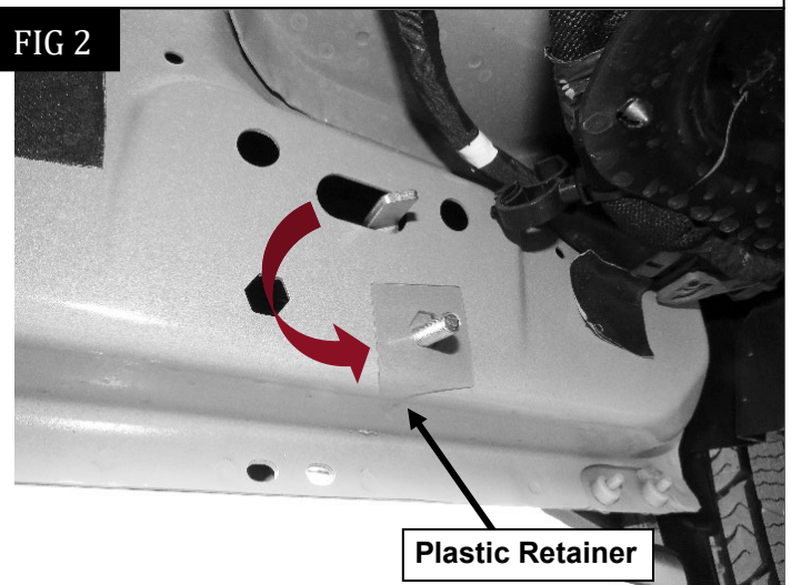
(Fig 2) Insert (1) 8mm Bolt Plate into the upper slot and line the threaded bolt up to the front hex hole, Thread (1) 8mm Plastic Retainer over the threads to hold it in place
