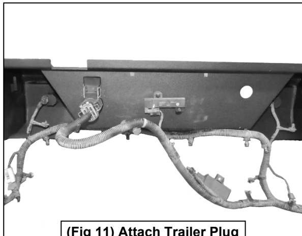
(Fig 11) Attach Trailer Plug and harness to bumper
