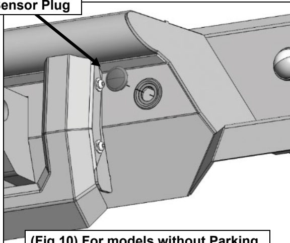
(Fig 10) For models without Parking Sensors, attach Plastic Plugs
