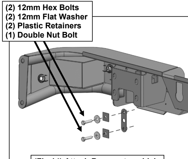
(Fig 14) Attach Bumper to vehicle
