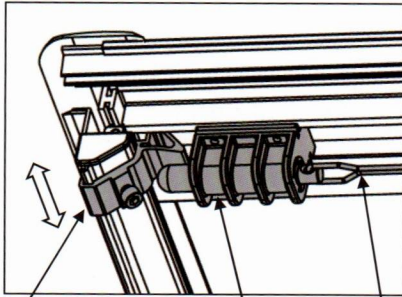
Locking Tongue(1-G)
