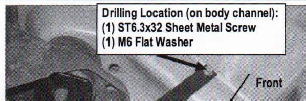
(Fig 4) Driver Front Support Bracket (DFS/PFS) Installed
