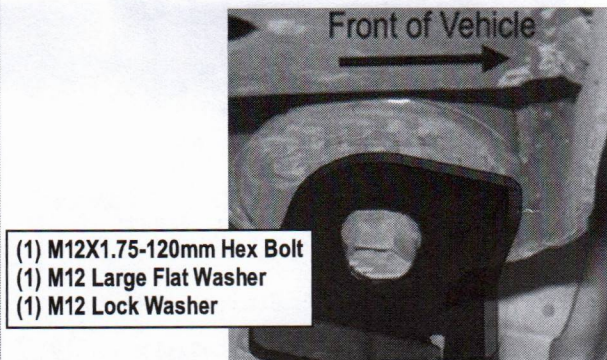
(Fig 6) Driver Side Rear Mounting Bracket (DRM) Installed
