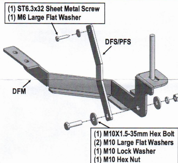
(Fig 3) Driver Front Support Brackets Installation
