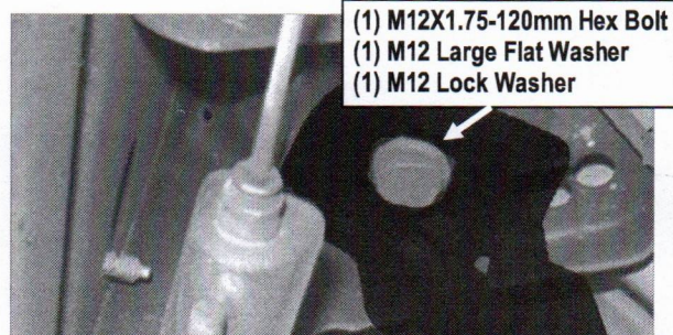
(Fig 2) Driver Front Mounting Bracket (DFM) Installed
