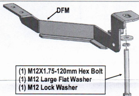
(Fig 1) Driver Front Mounting Bracket (DFM) Installation
