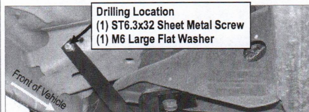
(Fig 7) Driver Side Rear Support Bracket (DRS/PRS) Installed
