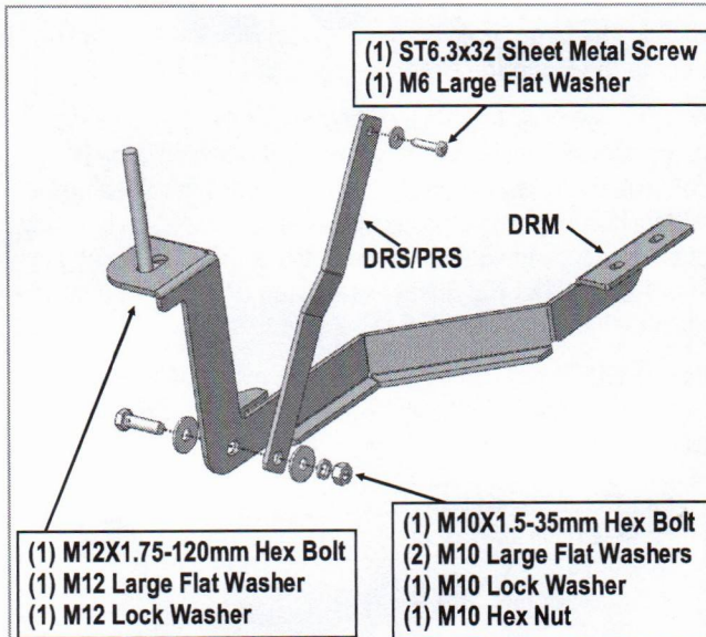
(Fig 5) Driver Side Rear Brackets Installation
