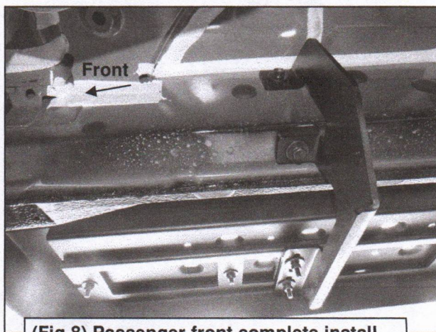
(Fig 8) Passenger front complete install
