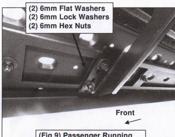
(Fig 9) Passenger Running Board attached to Bracket
