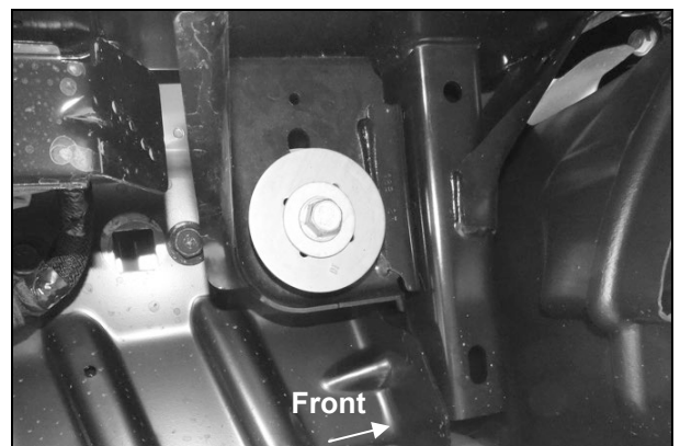
(Fig 4) Locate driver/left side front body mount
