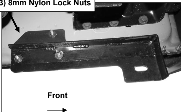
(Fig 3) Attach Bracket to the (3) studs
