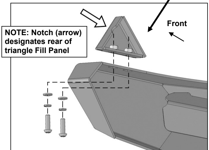
(Fig 17) Attach Driver/left side triangle Fill Panel to top corner of Bumper assembly
