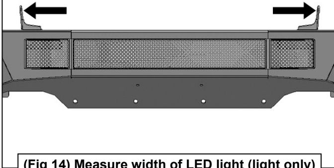
(Fig 14) Measure width of LED light (light only) before installation of Top Light Brackets
