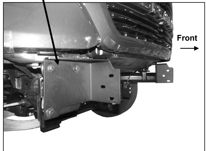
(Fig 11) Attach passenger/right Frame Mounting Bracket to end of frame
