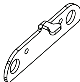
22 x2 Spacer (front drive linkage)
