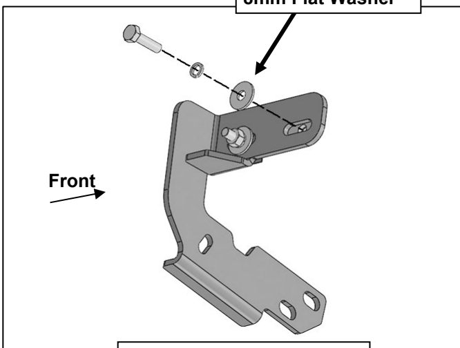
(Fig 7) Attach Bracket to threaded end of Bolt Plate
