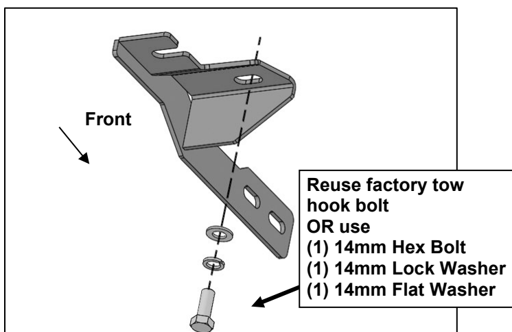
(Fig 18) Passenger/right side Frame Bracket attached to frame illustrated
