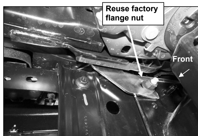
(Fig 13) Passenger/right side Rear Support Bracket attached to the back of the bumper bracket
