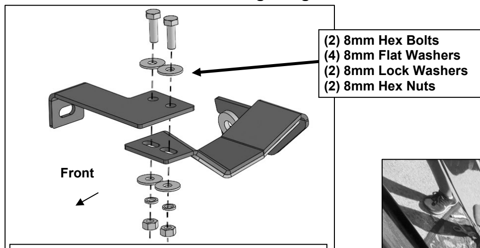
(Fig 14) Passenger/right side Front Support Bracket attached to the top of the Rear Bracket
