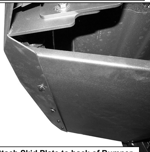
(Fig 4) Attach Skid Plate to back of Bumper
