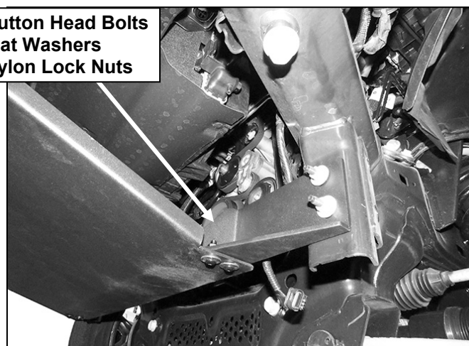
(Fig 6) Attach Skid Plate to Mounting Brackets
