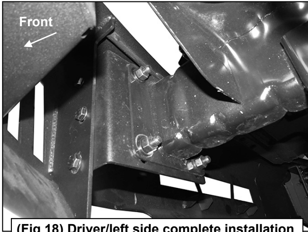
(Fig 18) Driver/left side complete installation
