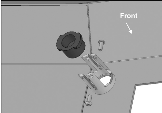
(Fig 9) Insert Plug into sleeve on back of bumper
