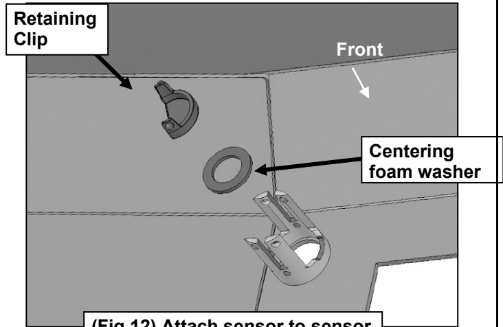
(Fig 12) Attach sensor to sensor sleeve on back of bumper
