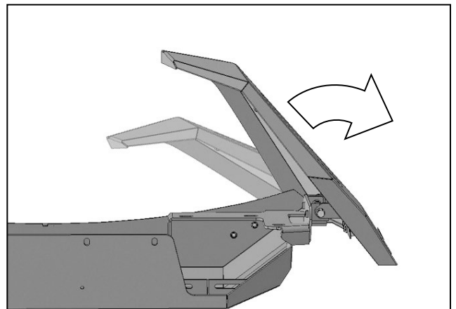
(Fig 8) Unfold outer Wings from center Bumper. Passenger/right side illustrated from below
