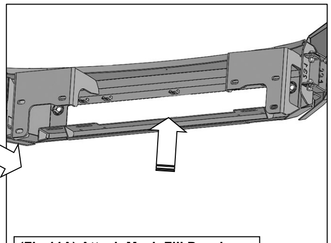
(Fig 11A) Attach Mesh Fill Panels as desired to fill unused openings for lights (lights not included).
