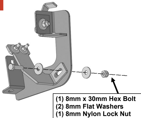
(Fig 7) Attach the Support Bracket to the Mounting Bracket
