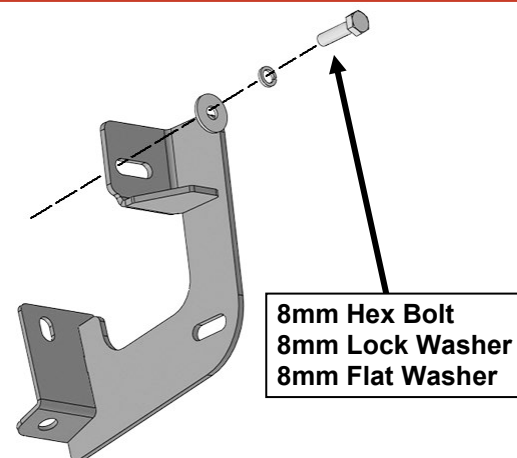
(Fig 5) Attach Driver/Left Mounting Bracket to factory installed threaded inserts
