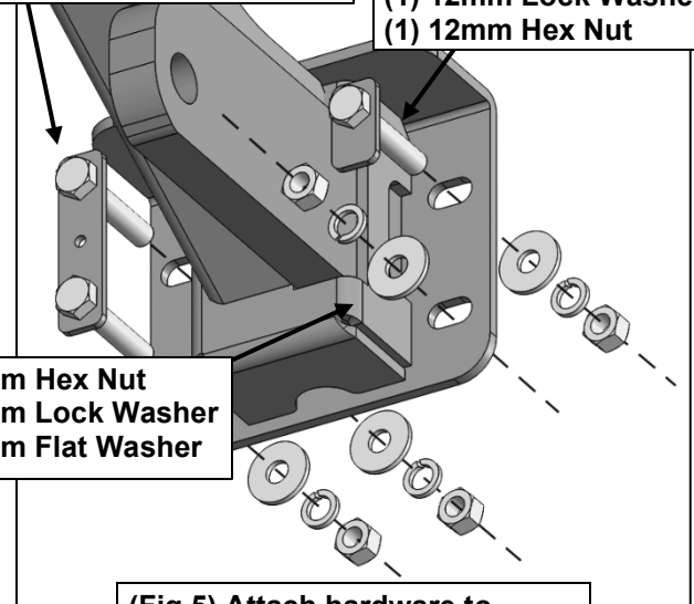
(Fig 5) Attach hardware to connect Winch Tray to Bumper
