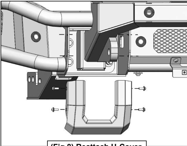
(Fig 8) Reattach U-Cover
