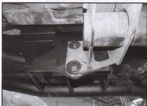
(Fig 19) Passenger side of the Rear Bumper attached to the factory hitch
