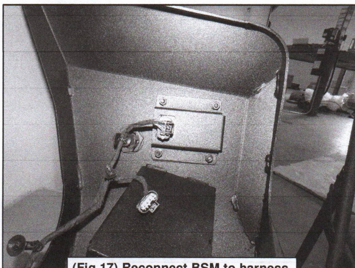
(Fig 17) Reconnect BSM to harness
