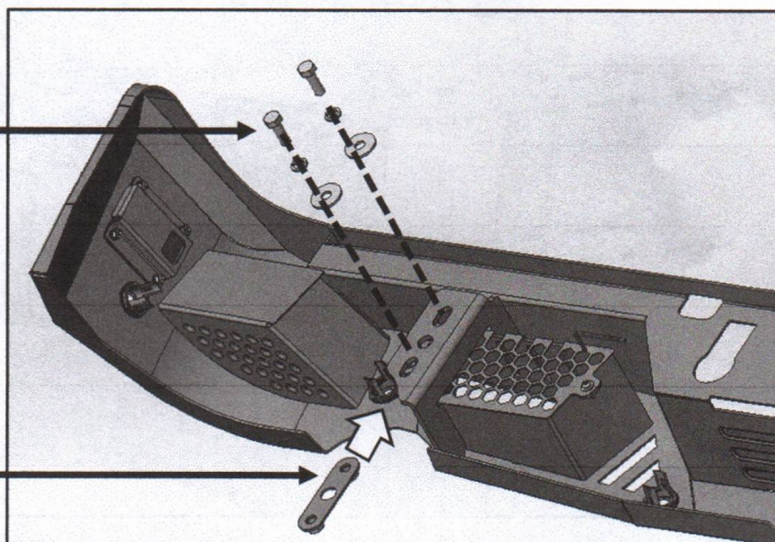
(Fig 18) With assistance, slide Nut Plate through the back of the Bumper
