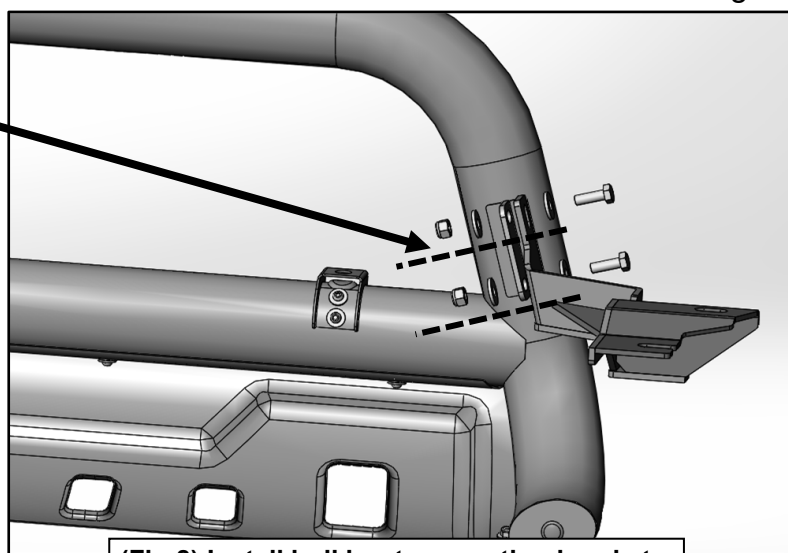
(Fig 8) Install bull bar to mounting brackets
