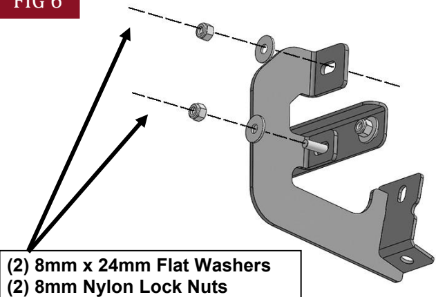
(Fig 6) Attach (1) Center Mounting Bracket ( #3 ) to the upper threaded stud and Support Bracket
