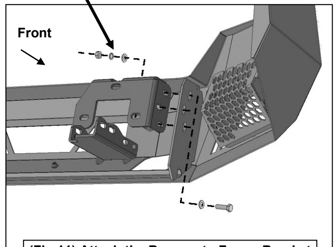
(Fig 11) Attach the Bumper to Frame Bracket
