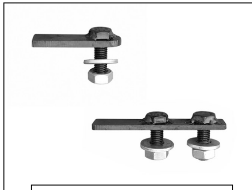
(Fig 7) 12mm Single Bolt Plate and 12mm Double Bolt Plate
