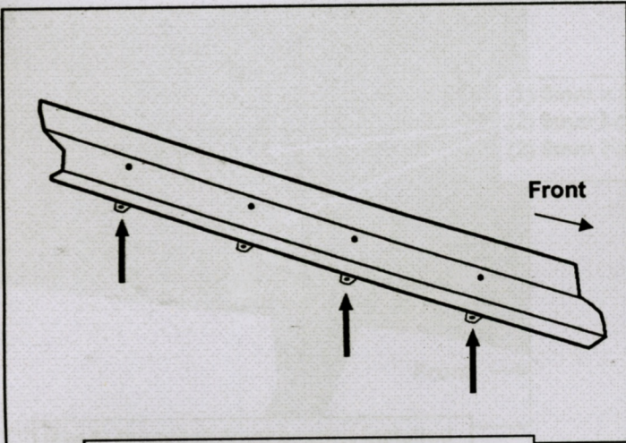
(Fig 1) Driver side (3) mounting locations
