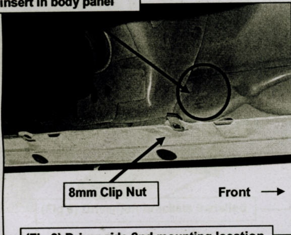
8mm Clip Nut (Fig 3) Driver side 2nd mounting location
