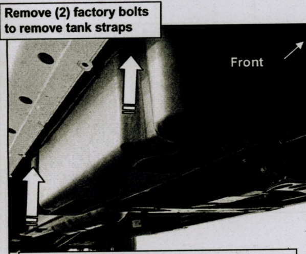
(Fig 10) Passenger side DEF tank and cover
