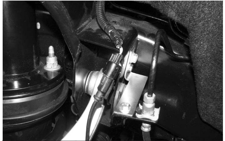
FIGURE 68 - STEP 45
