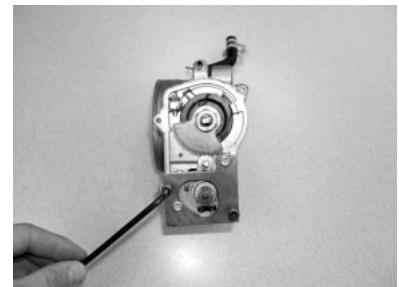
Assembly Step 5
