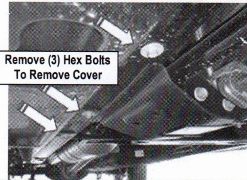
(Fig 8) 07-16 Passenger Side Front With DEF Tank Cover
