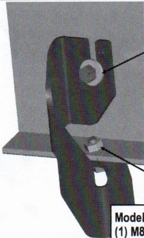
(Fig 11) Passenger Front Mounting Bracket Installed (example)
