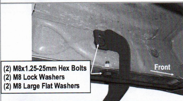
(Fig 5) Driver Front Mounting Bracket Assembly
