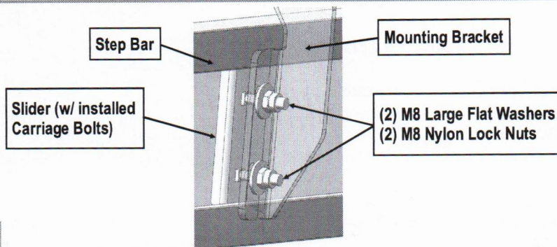
(Fig 7) Step Bar Installation
