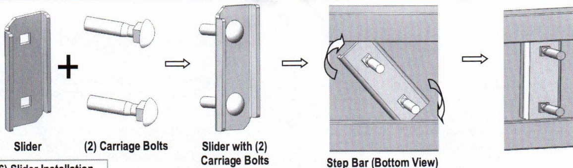
(Fig 6) Slider Installation
