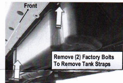
(Fig 9) Passenger side 07-16 DEF tank and cover
