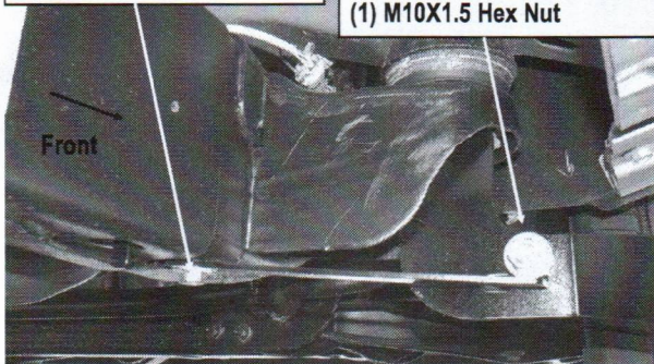
(Fig 4) Passenger Side Front Support Bracket Installed (1500 Models )
