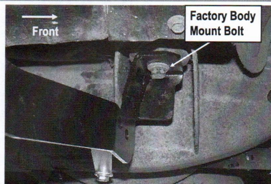
(Fig 2) Passenger Front Mounting Bracket Installed
