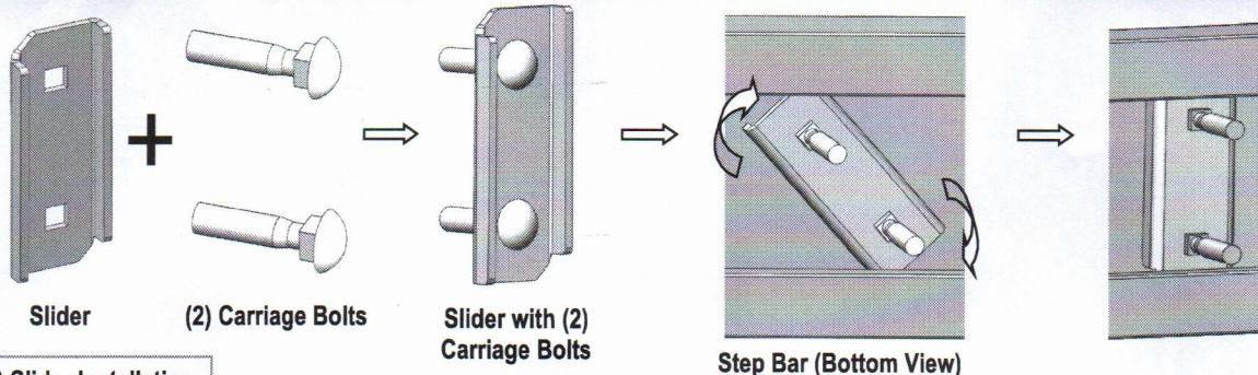
(Fig 9) Slider Installation
