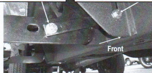
(Fig 6) Passenger Center Bracket Installed (1500 Models)
