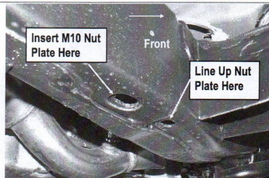
(Fig 3) Passenger Front Support Bracket Mounting Location
