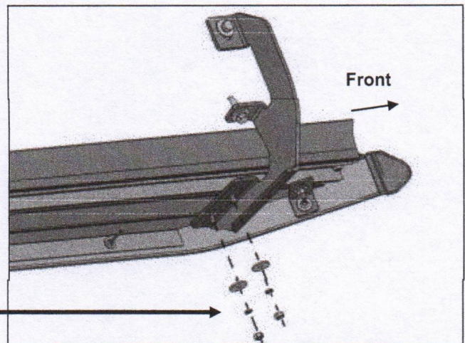
(Fig 8) Attach Running Board to Brackets
