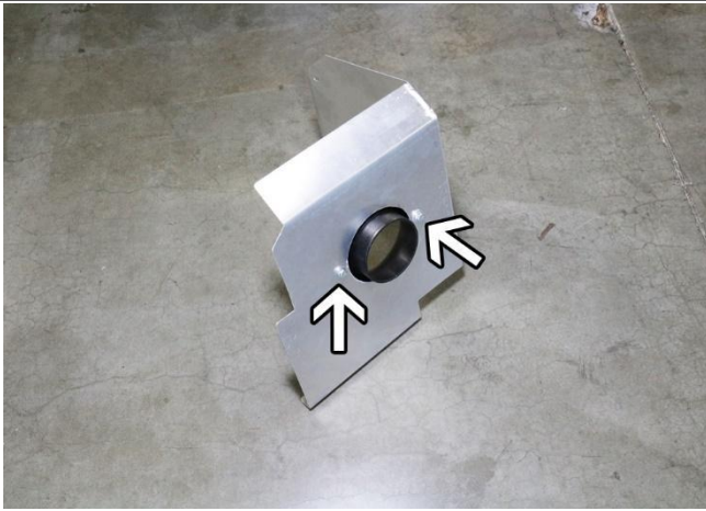
12. Install and secure the velocity stack onto the heat shield using two 6mm x 12mm and washers provided in the hardware kit.
