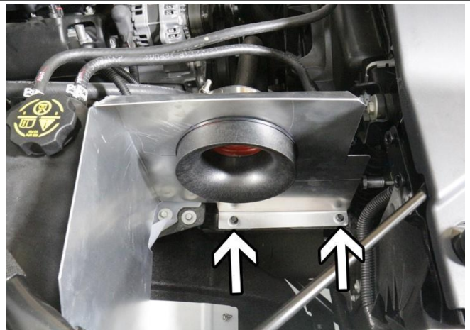
15. Install the heatshield into the vehicle. Using the stock mounting holes from the air box tray, match the slots from the heatshield and secure the heatshield using two 6mm x 20mm bolts and washers.
