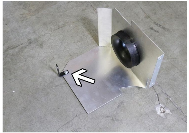
13. Install the provided "L" bracket onto the heatshield using a 6mm x 12mm bolt, nut, and two washers.
