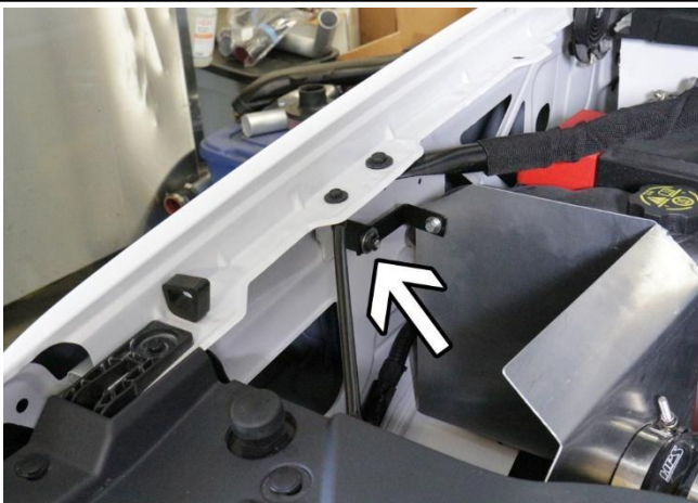
16. Secure the heat shield bracket onto the vibration mount.
