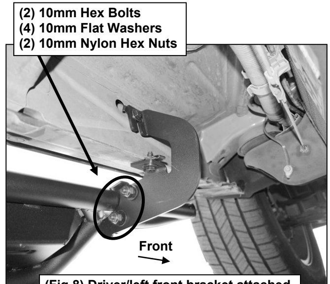
(Fig 8) Driver/left front bracket attached to driver side Running Board
