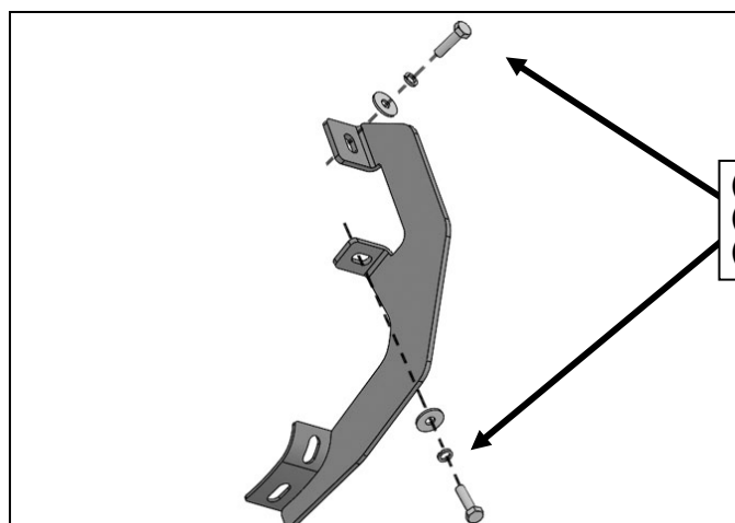
(Fig 3) Mounting Bracket illustration
