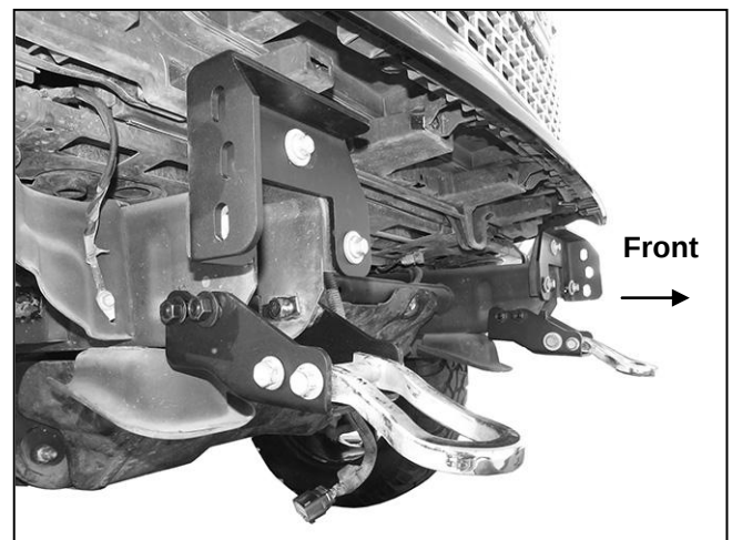
(Fig 10) Brackets and tow hooks installed
