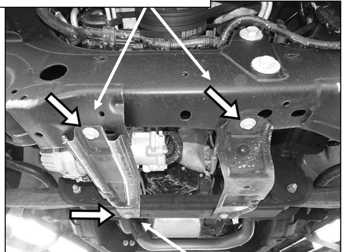
(Fig 2) Loosen the (1) hex bolt attaching the passenger side skid plate to the rear crossmember
