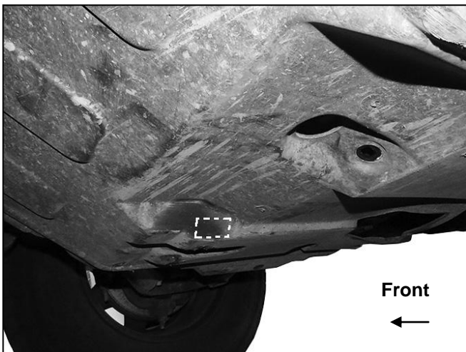
(Fig 3) Mark the splash guard to cut for Bracket clearance. Note insert flat passenger side of Bracket through slot and between skid plate and crossmember
