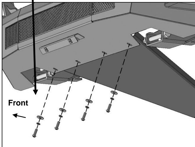
(Fig 6) Attach LD2 Skid Plate to back of Bumper
