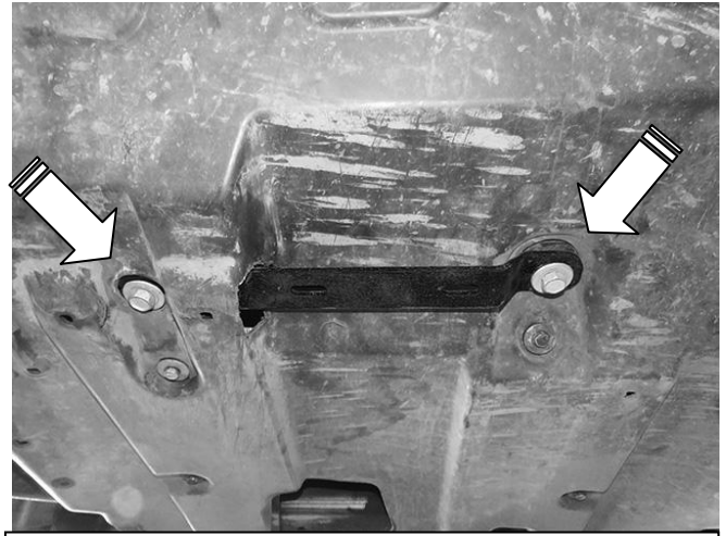
(Fig 5) Insert flat end of Bracket through hole cut in splash guard. Insert end of Bracket between steel skid plate and crossmember (behind splash guard). Reuse factory hex bolts (arrows) to attach Bracket
