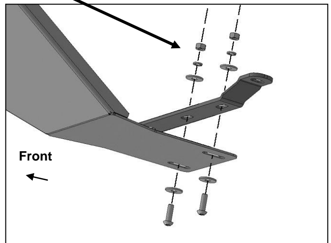
(Fig 7) Attach LD2 Skid Plate to Rear Bracket
