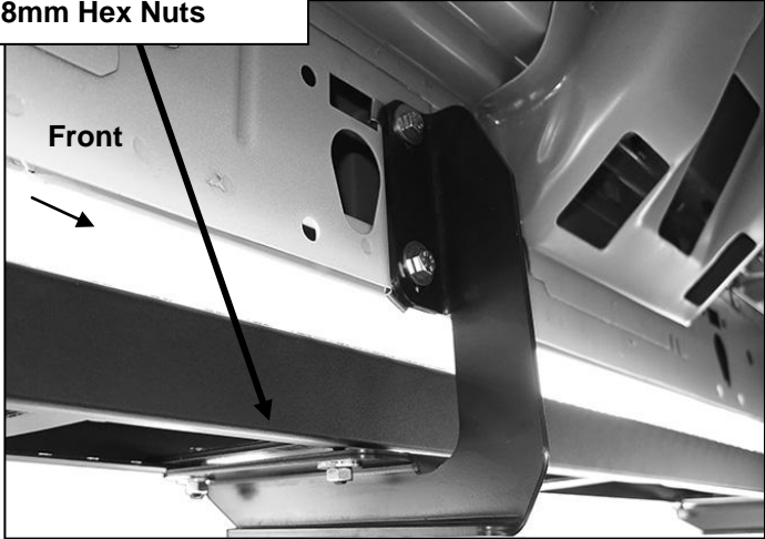
(Fig 11) Driver/left center Mounting Bracket installed
