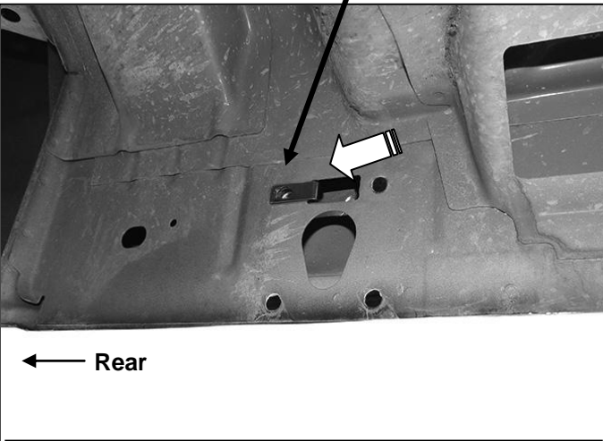
(Fig 6) Driver/left rear Mounting Bracket location
