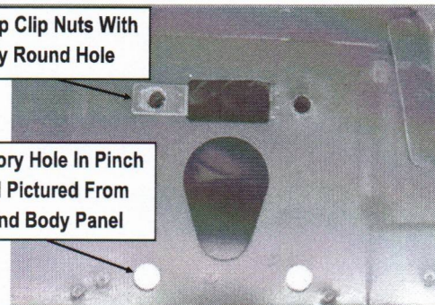
(Fig 3) M10 Clip Nut Installed
