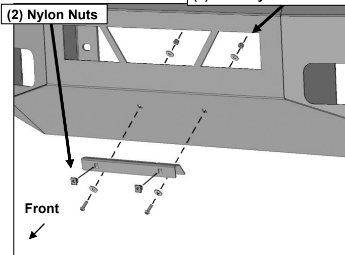
(Fig 10) Attach License Plate Bracket to Bumper
