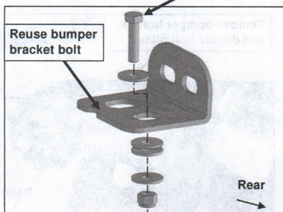
(Fig 9) 2023+ models with built in receiver hitch. Reuse the factory hardware to attach the front slot in the Bracket. Use the included 10mm hardware to attach the rear mounting slot in the Support Bracket
