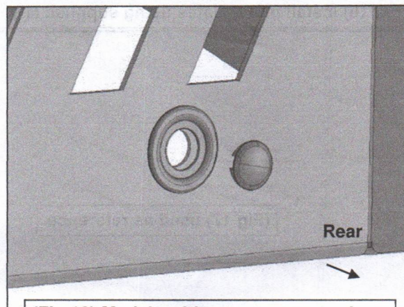
(Fig 13) Models without sensors, push sensor hole plugs into mounts
