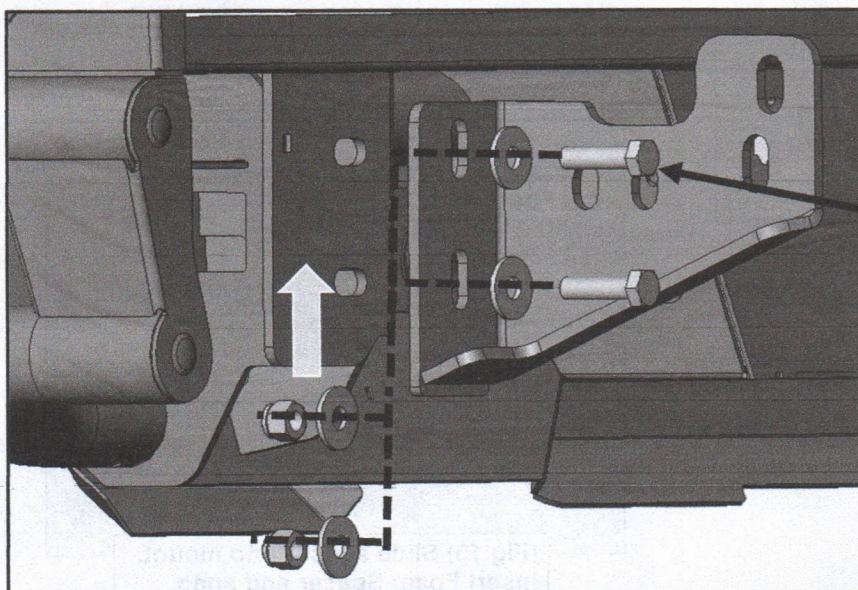
(Fig 18) Install the bumper to the mounting brackets using supplied HW
