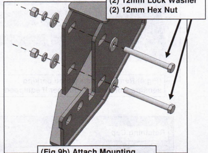
(Fig 9b) Attach Mounting Bracket to mounting location
