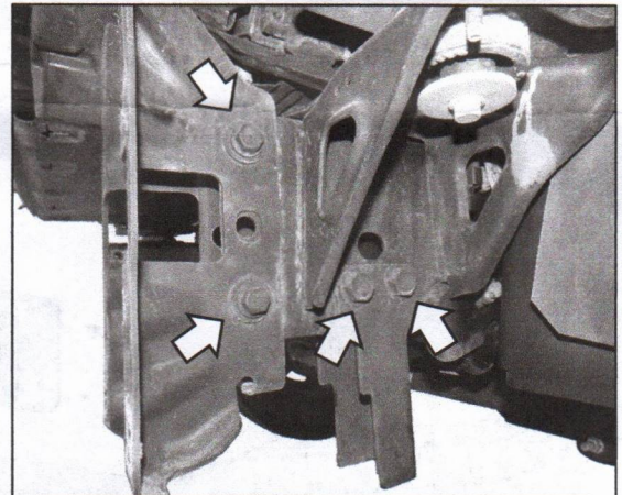
(Fig 2) Remove hardware from factory bumper to clear mounting location
