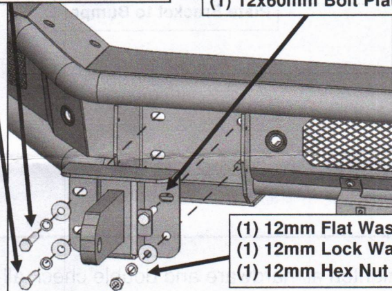
(Fig 15) Attach Tow Hook to Bumper
