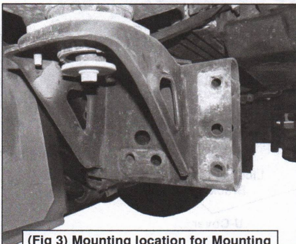
(Fig 3) Mounting location for Mounting Bracket (Passenger/Right pictured)
