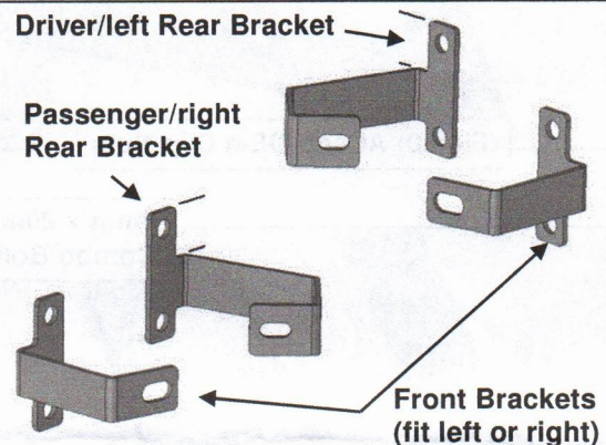
(Fig 16) Select driver/left CTA Brackets
