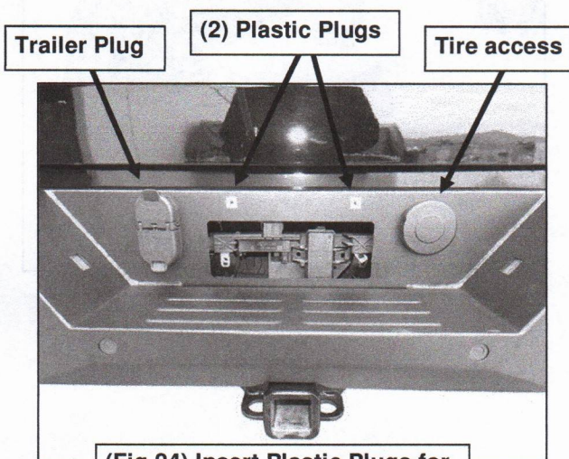
(Fig 24) Insert Plastic Plugs for license plate, and install Trailer Plug and Tire Access Plug
