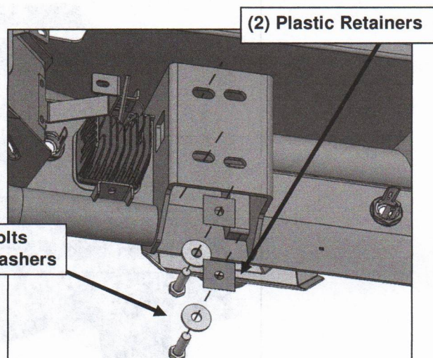
(Fig 28) Attach (2) 12mm Hex Bolts to Bumper. For 1500 models, use outer slots. For 2500-3500 models, use inner slots.
