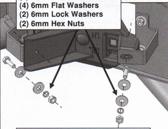
(Fig 19) Attach sensor to Brackets
