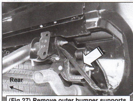
(Fig 27) Remove outer bumper supports from both sides of frame (arrow)
