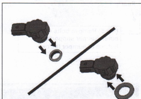
(Fig 11) Models with parking sensors, remove silicone seal from sensor. Slide Foam Seal over end of sensor (arrow)
