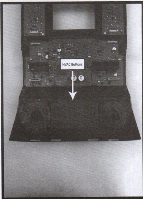
10. Remove HVAC buttons (make sure the rubber button pad comes with it). Set aside for later use.
