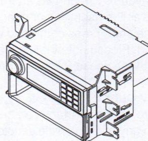
Mount radio to brackets using supplied screws
