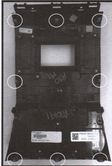
2. Remove (8) orange clips from factory dash panel using a small flathead screwdriver. Set aside for later use.
