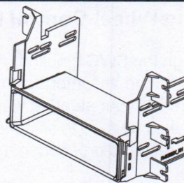
Attach included pocket to bottom of kit brackets
