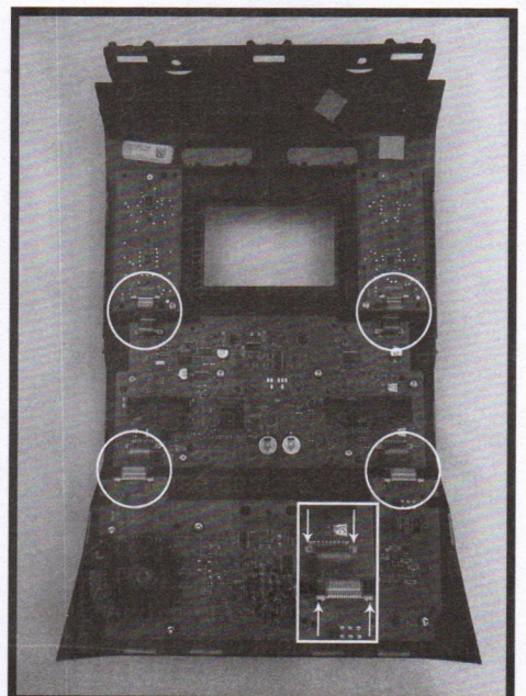
6. Remove (4) ribbon cables from circuit boards on factory dash panel by pulling out on the white release tabs.
