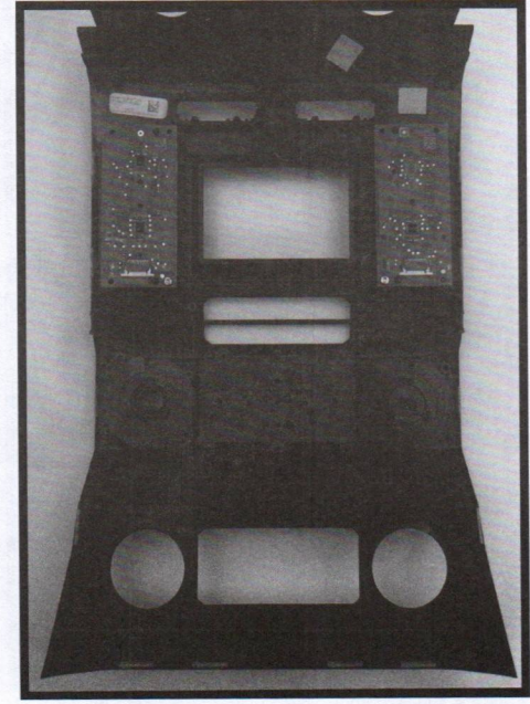
12. Remove middle circuit board and set aside for later use. Make sure that the rubber pads for the buttons and knobs stay behind with the factory dash panel.
