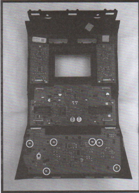
7. Remove (6) T10 16mm screws from bottom circuit board. Set aside for later use.
