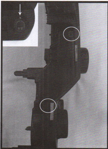
4. Make sure that the white line on the temperature control knob is centered at the top. Remove back of factory dash panel by releasing the locking tabs on each side.
