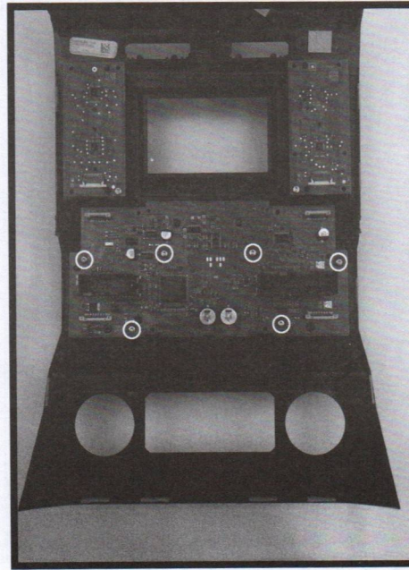
11. Remove (6) T10 16mm screws from middle circuit board. Set (2) aside with the (6) from step 7 for later use.
