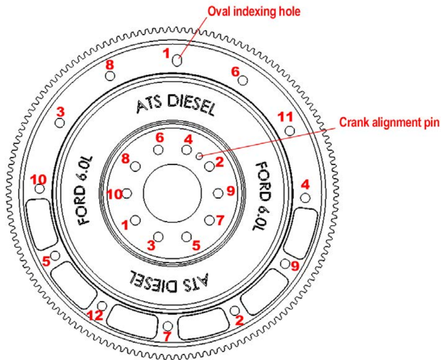
Figure 1: Oval Index Hole and Torque Sequence
