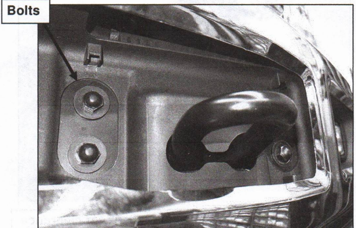
(Fig 4) Remove bumper bolts (driver side pictured)
