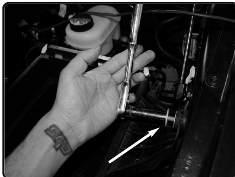
5. Loosen the bolt holding in the bottom of the airbox using 13mm socket or wrench.
