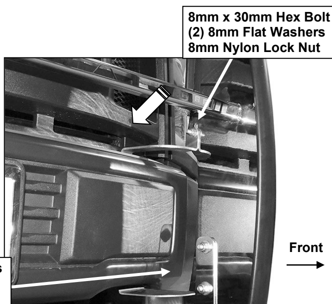
(Fig 24) 2015-17 models: Complete installation
