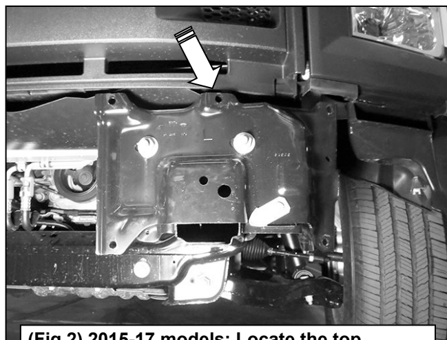
(Fig 2) 2015-17 models: Locate the top bumper bolts. Remove the driver side middle bolt (see arrow-bumper pictured removed for reference only-do not remove bumper)
