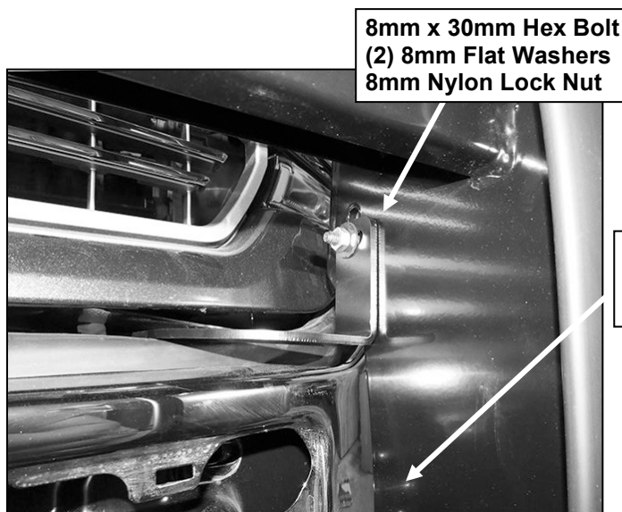
(Fig 25) 2018 models: Complete installation
