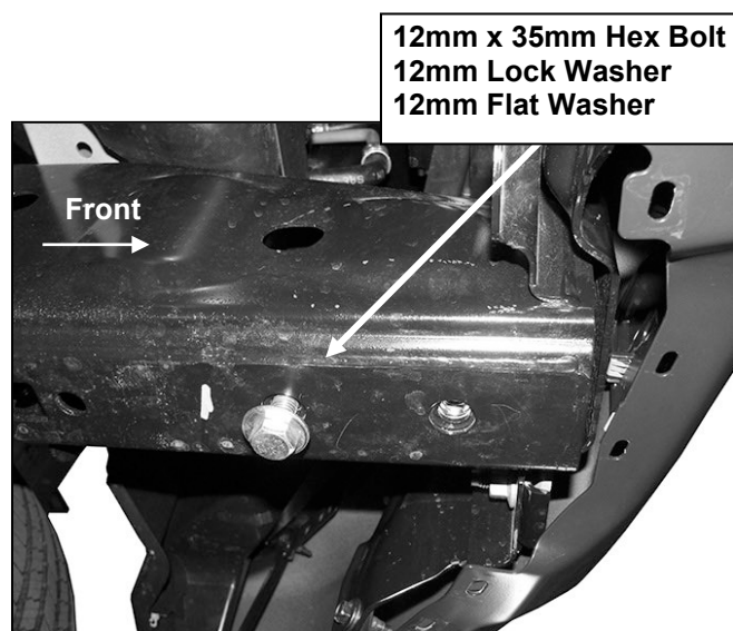
(Fig 14) Use a Hex Bolt to line up the Nut Plate
